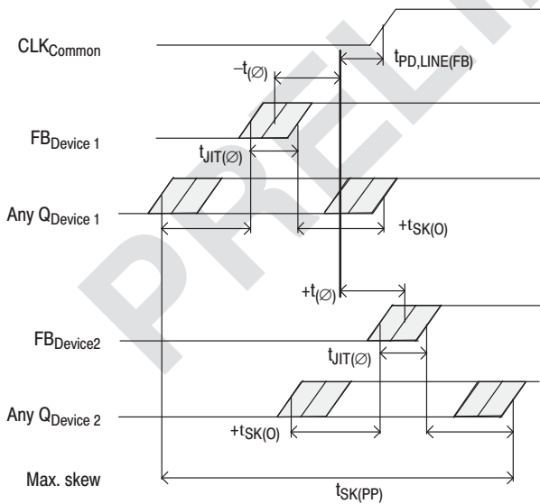
Complementary signals are not shown. Signal references level is the differential voltage crosspoint V_X
