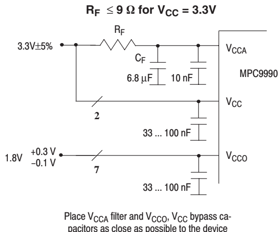
Figure 9. Recommended Power Supply Filter
