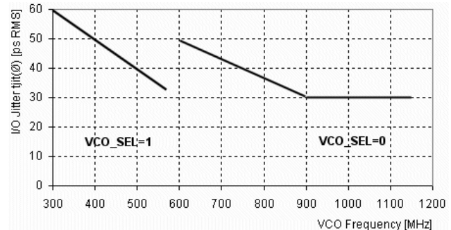
Figure 8. Max. I/O Jitter versus frequency
